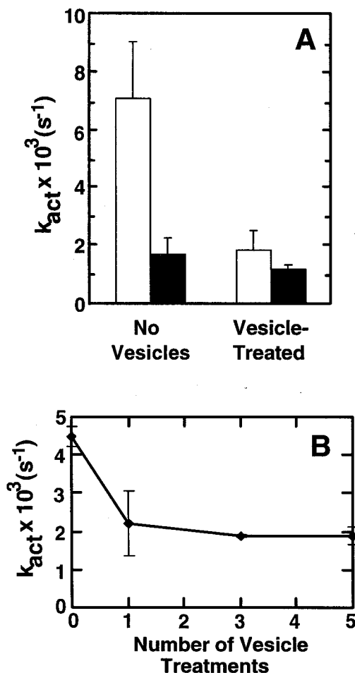
FIGURE 4 Complete removal of retinal-oxime eliminates NH_2OH sensitivity. (A) Treatment with sonicated PC vesicles reduces k_{act} and nearly eliminates NH_2OH sensitivity. Membranes were washed twice with pH assay buffer 2 plus 100 mM NH_2OH , followed by two washes of buffer alone. "Vesicle-treated" membranes were then washed with a sevenfold molar excess (vesicle lipid/ROS lipid) of PC vesicles (12 h incubation with vesicles), and "No vesicles" membranes were washed with buffer alone. Membranes were assayed in the presence of 150 mM NaCl (empty bars) or 150 mM NH_2OH (filled bars). pH assays were carried out on membranes (8 \mu M R) reconstituted with G_t and PDE extracts in pH assay buffer 2 (with NH_2OH-HCl or NaCl substituted for KCl). Assays were initiated by adding 32 \mu M GTP \gamma S and cGMP to an initial concentration of 8 mM. For the "No vesicle" experiment with added NH_2OH (filled bar), n = 3 , and n = 4 for all other conditions. (B) Simultaneous exposure to vesicles and NH_2OH results in the lowest k_{act} and complete elimination of NH_2OH sensitivity. Membranes were washed twice with pH assay buffer 2 plus 100 mM NH_2OH , followed by two washes of buffer alone before being treated the indicated number of times with a 10-fold lipid:lipid molar excess of PC vesicles and 100 mM NH_2OH simultaneously (45-min incubations). Assays were conducted in the same buffer, except that NaCl was substituted for KCl. Membranes (20 \mu M R) were reconstituted with PDE and G_t , and hydrolysis of 8 mM cGMP was monitored after the addition of GTP \gamma S (32 \mu M ). Assays were carried out with additional 20 mM NH_2OH-HCl , and the NaCl concentration was reduced to 130 mM to keep the assay conditions isotonic. After three vesicle/ NH_2OH treatments, retinal-oxime levels were below our spectroscopic detection limits. Points are averages of duplicate or triplicate assays \pm standard deviation.
